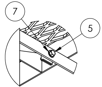
DETAIL B SCALE 1 : 6
