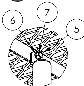
DETAIL C SCALE 1 : 6
