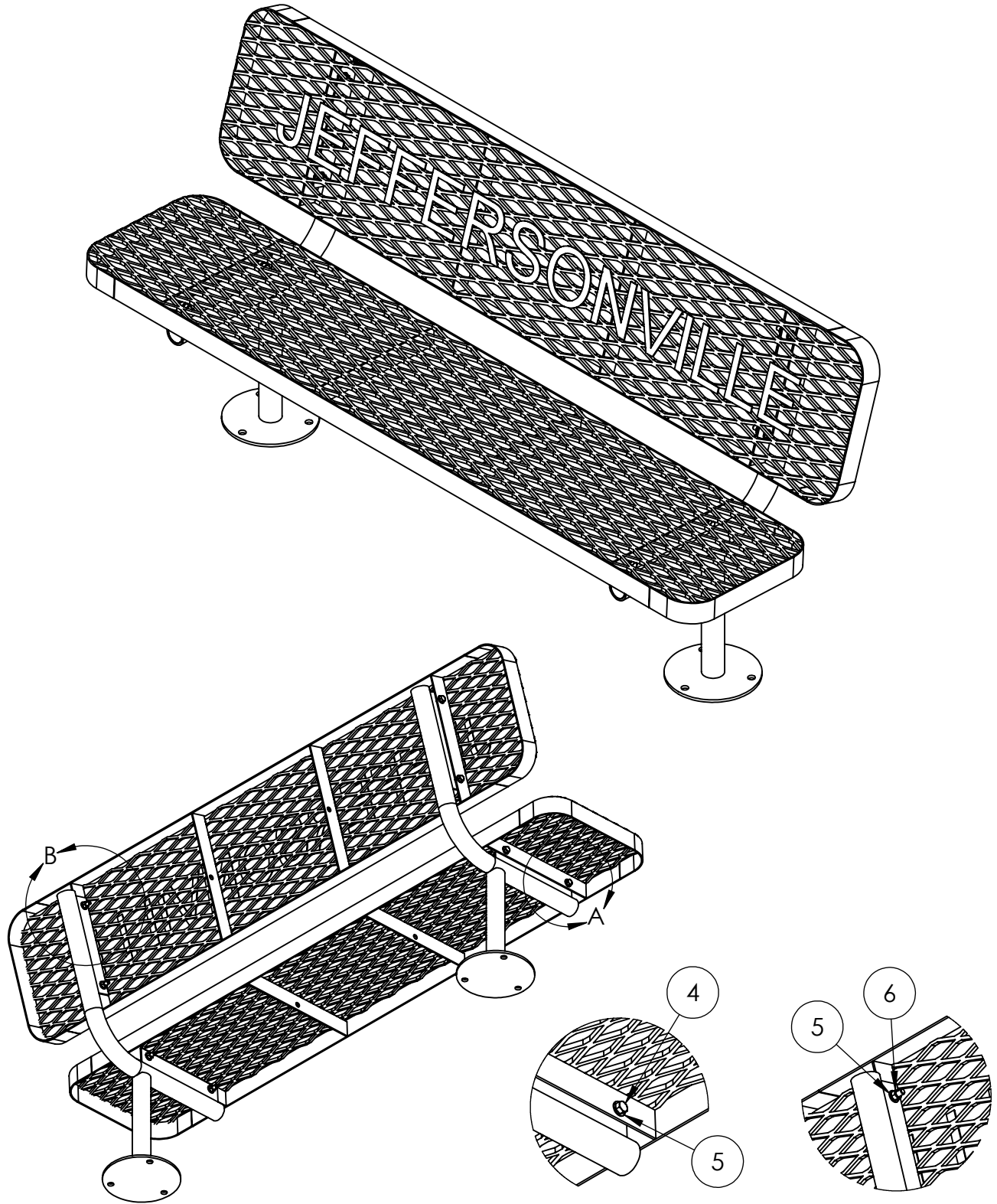
DETAIL A
